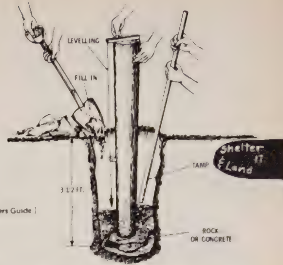
1. A method of erecting a post. Note the large rock or concrete at bottom of the hole. The post is leveled from all angles with a slumb bar.
